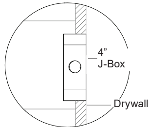
J-Box Positioning
