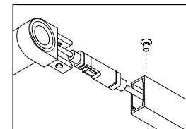
Connect rail wire harness to power wire harness
