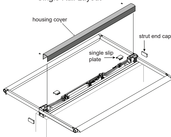
Single Rail Layout
